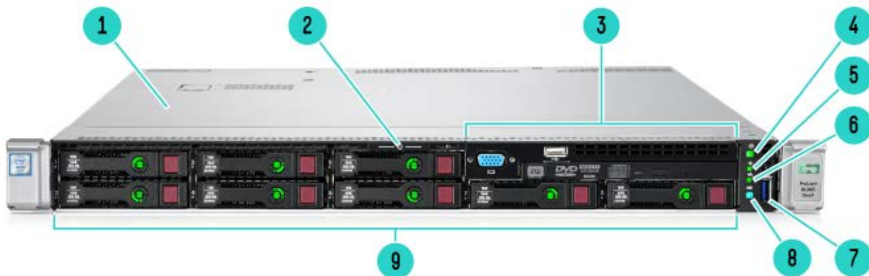
Front View
